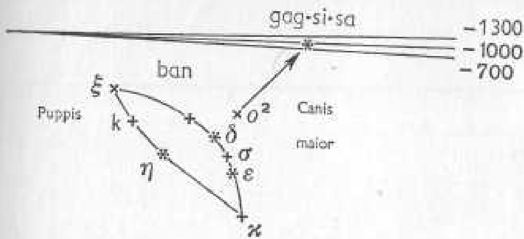
The Mesopotamian constellation of Bow and Arrow (𒍪BAN and 𒍪KAKSIDI, or gag-si-sa), as reconstructed on the evidence of astronomical cuneiform texts; gag-si-sa/KAKSIDI is Sirius, the "Arrow-Star."
